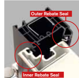
Double Rebate ApeerModo's double rebate system adds additional draught protection by creating an internal secondary rebated seal.
