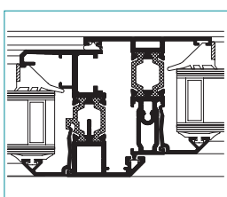
Mullion/vent
