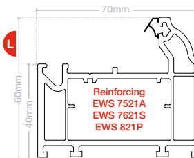
Main frame EWS 7721
