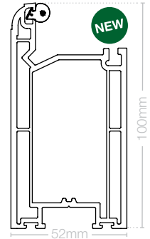
charisma classic Deep bottom rail VSW004
