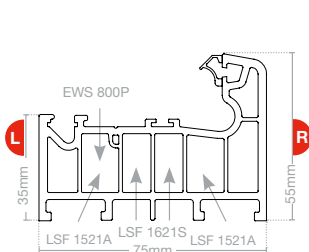
Main frame LSF 1021
