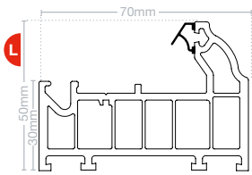
Thermalogik frame EWS 7701 Reinforcing EWS 800P
