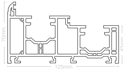
Frame VSW001
