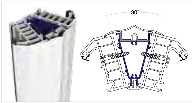
Bay post assembly 150° angle
