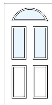
The Winstor Half moon cassettes R279mm x 250mm Mid panel cassettes 202mm x 578mm
