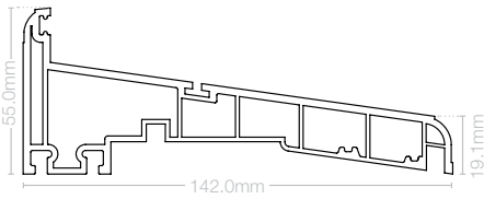
Ovolo cill adaptor VSW009
