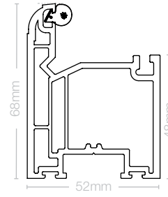
Medium bottom sash VSW003
