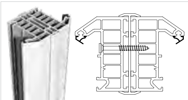
PVC-U butt joint assembly
