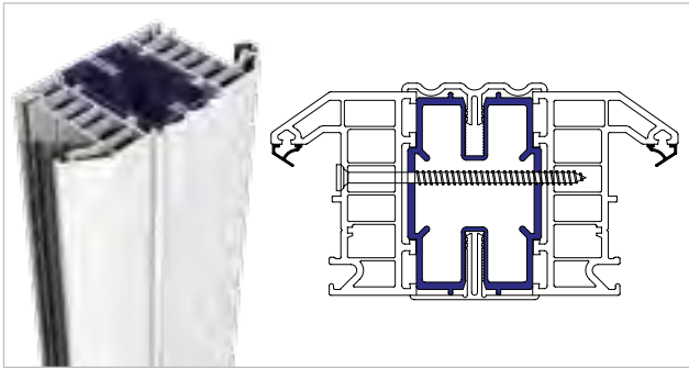
Structural butt joint assembly with sculptured trim
