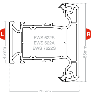
Intermediate Transom T LSF 1022
