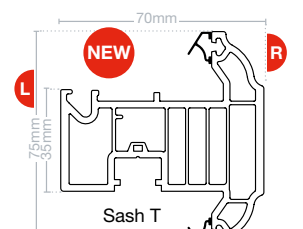
NEW Sash T EWS 7708 Reinforcing EWS 800P
