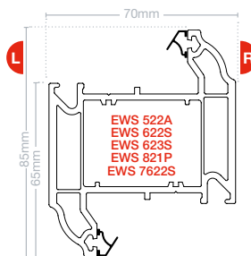
Intermediate transom Z EWS 7723
