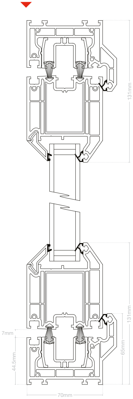
Vertical (open in)
