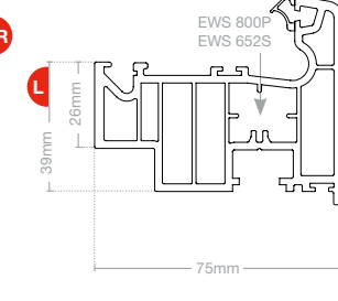
Reversible / Flush sash LSF 1008
