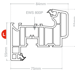
Tilt & turn flush sash LSF 1007
