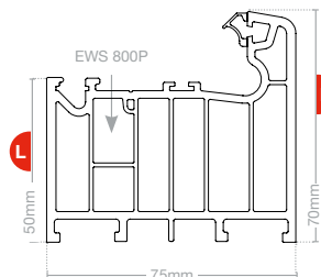
Large main frame LSF 1006
