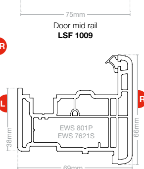
French door mullion LSF 1016
