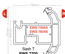
Sash T EWS 7705
