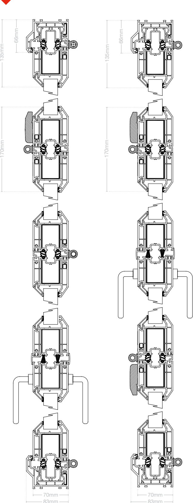
Horizontal (open out)
