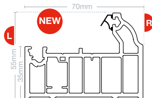
NEW Slim outer frame EWS 7720 Reinforcing EWS 800P
