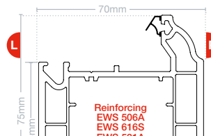
Large main frame EWS 7706
