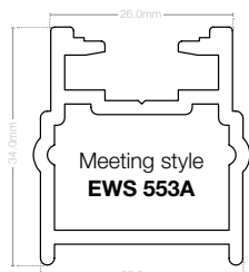
Cill reinforcement EWS 519A
